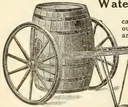
Water Truck as used with Barrel.
